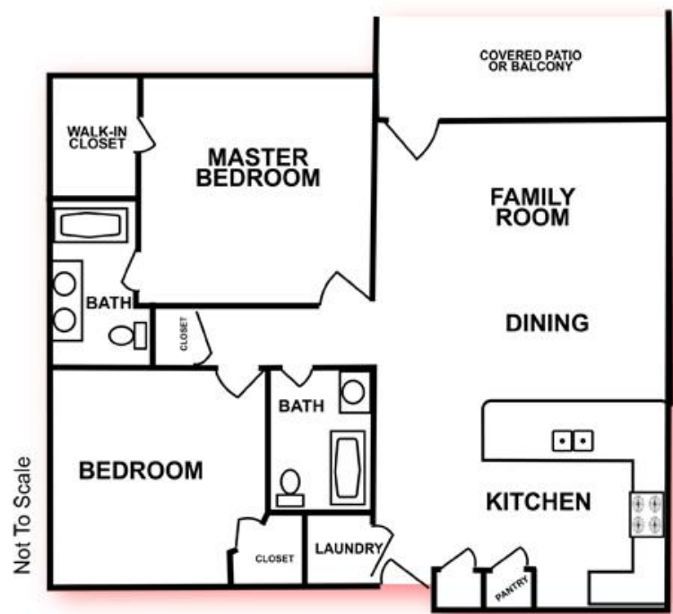
Milano Plan ±1,114 Sq.Ft.
