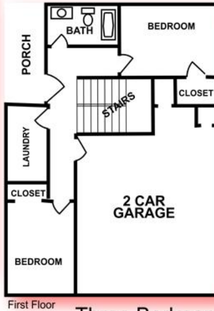
Three Bedroom ±1,545 Sq.Ft./ Buildings A&B
